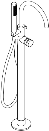
Free-standing bath mixer D 181 H 1012 mm Monocomando vasca a pavimento P 181 H 1012 mm
